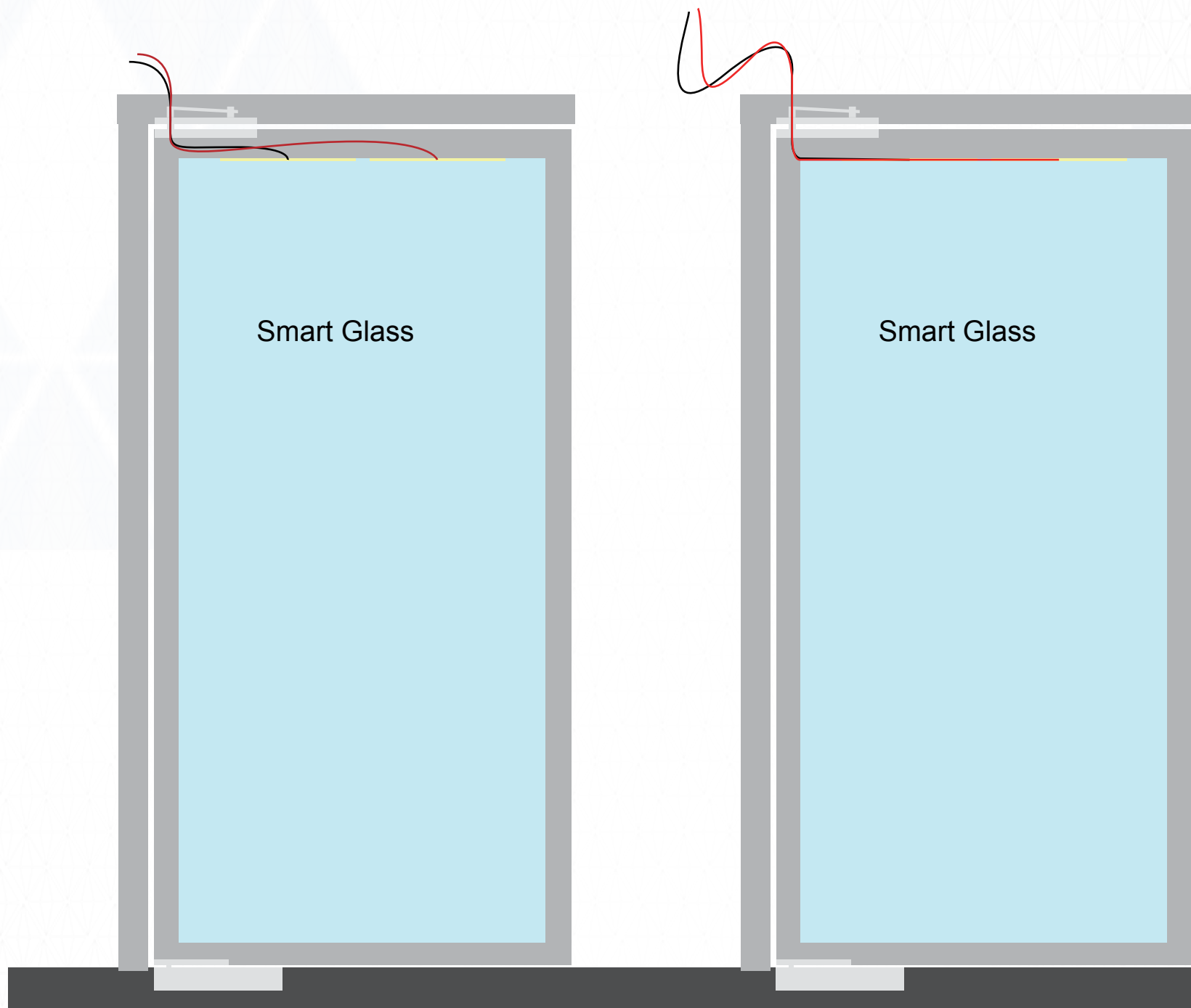
Connection of glass door clamp
